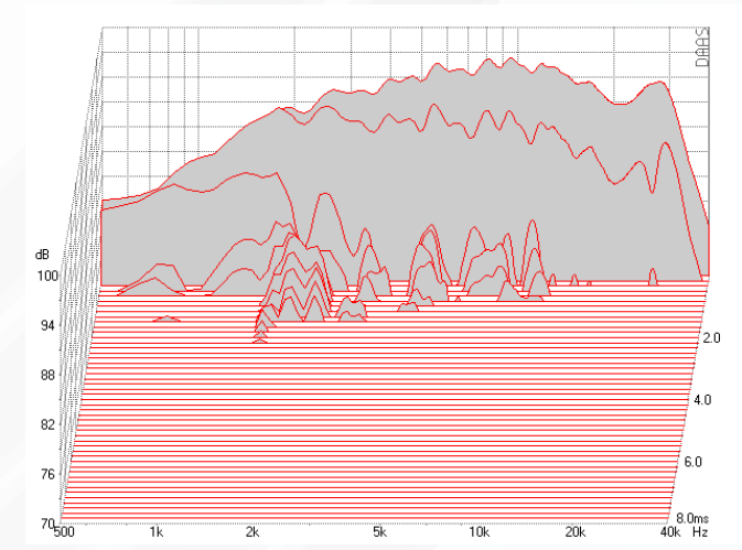
Waterfall
