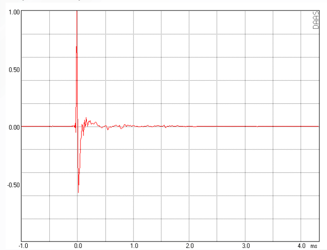
Impulse Response
